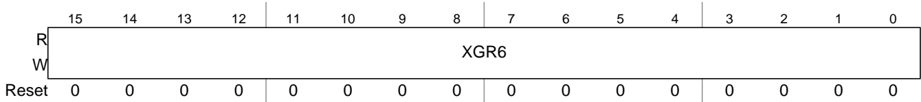
Figure 14-20. XGATE Register 6 (XGR6)
